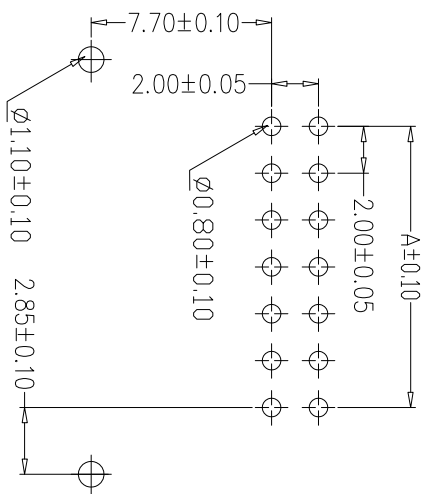
PCB LAYOUT
